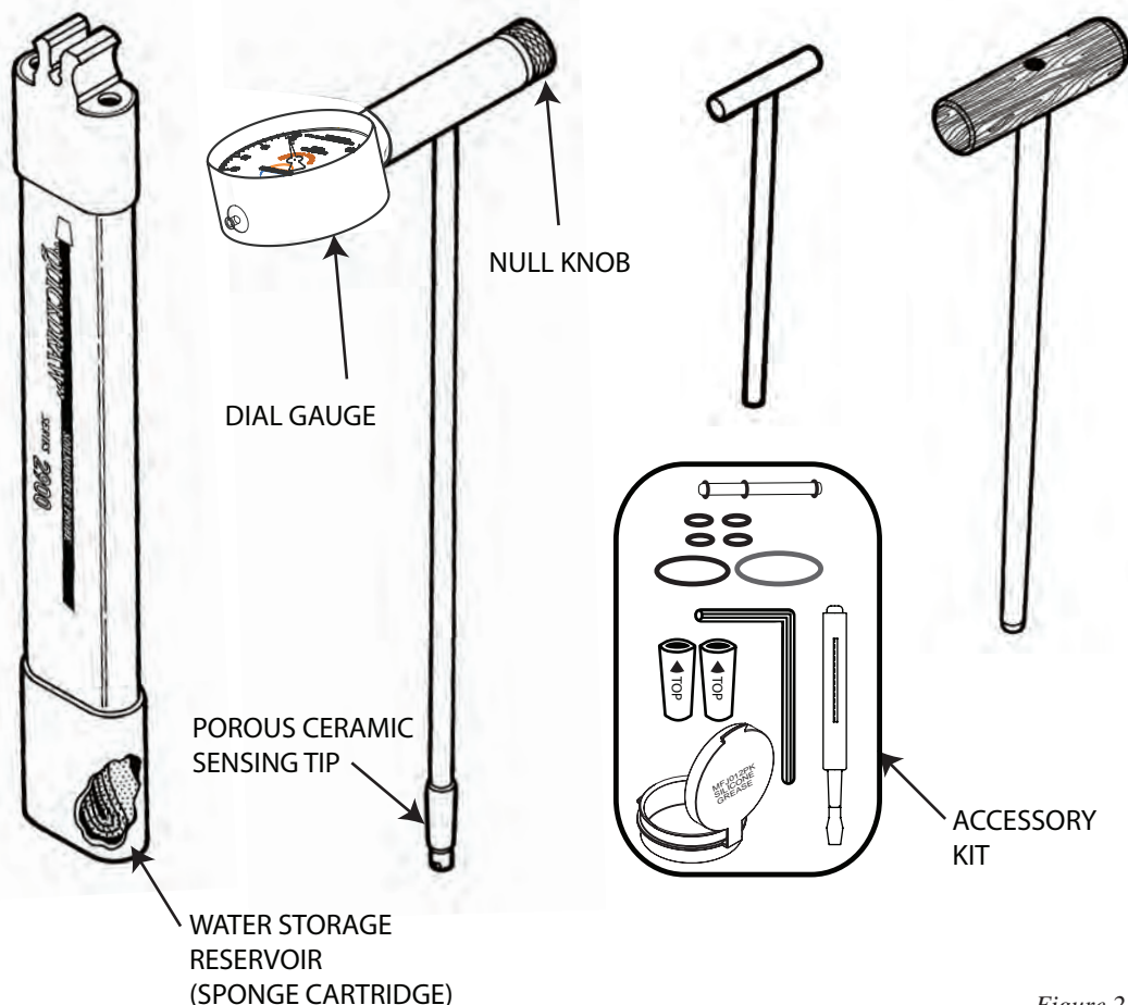
Figure 2 - 2900K1 Parts
