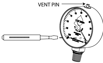
Figure 4 - Venting and adjusting the gauge
