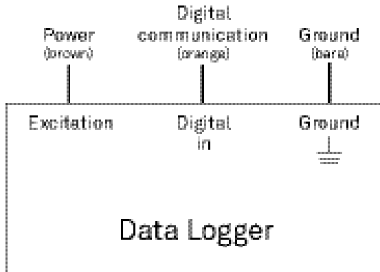
Figure 3 Wiring diagram
